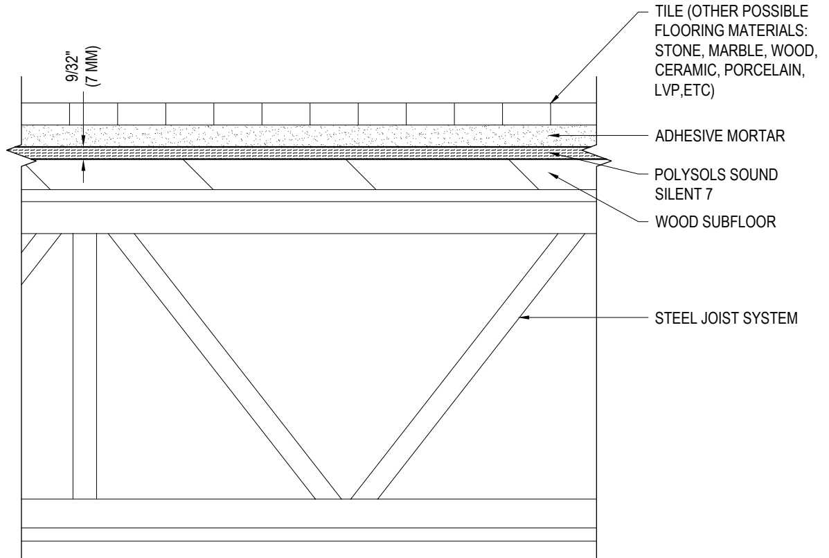
SECTION FLOORING ACOUSTICAL UNDERLAYMENT POLYSOLS SOUND SILENT 7 ON STEEL JOIST SYSTEM
